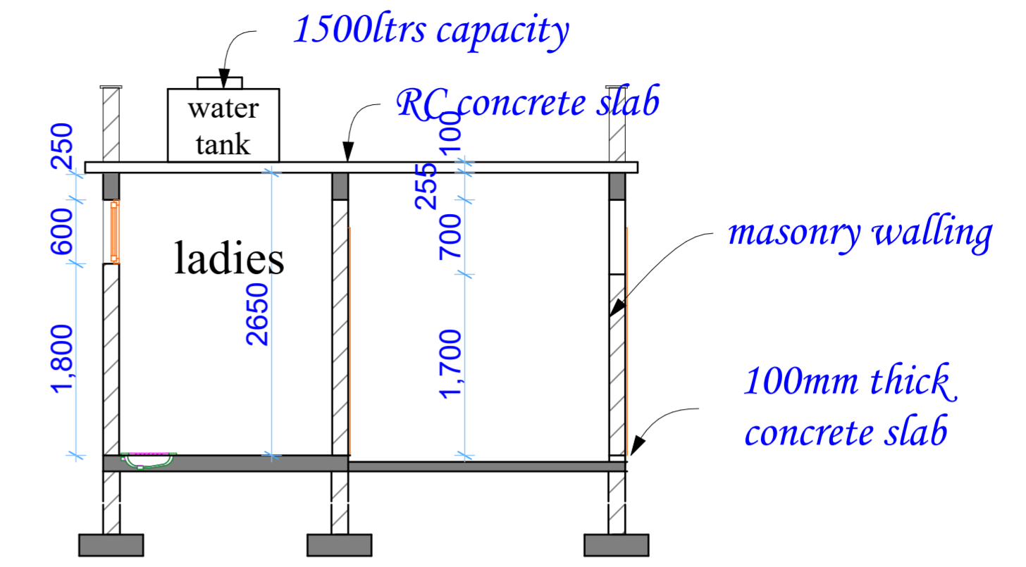
Section X-X scale 1;100
